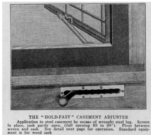
The “Holdfast” Adjuster
